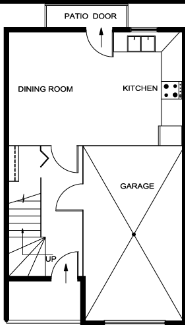
HUNTER STREET CHALET TOWNHOUSE MAIN FLOOR PLAN AREA = 660 SQUARE FEET
