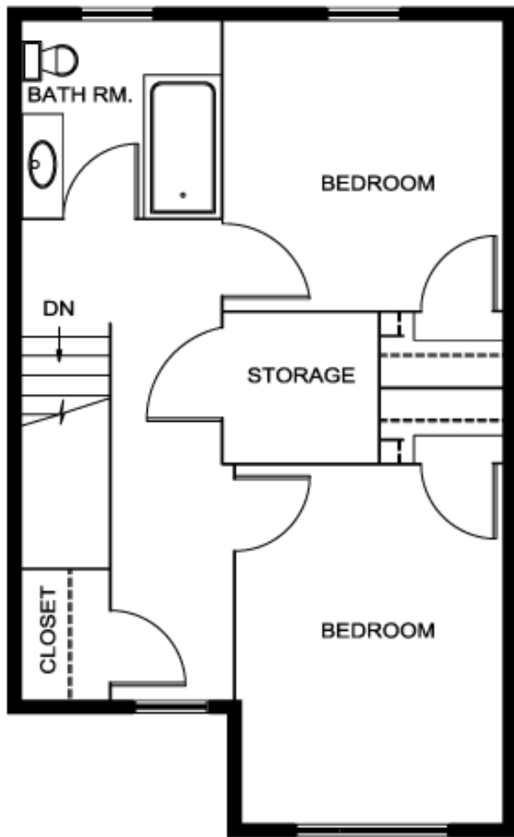
HUNTER STREET CHALET TOWNHOUSE THIRD FLOOR PLAN AREA = 615 SQUARE FEET
